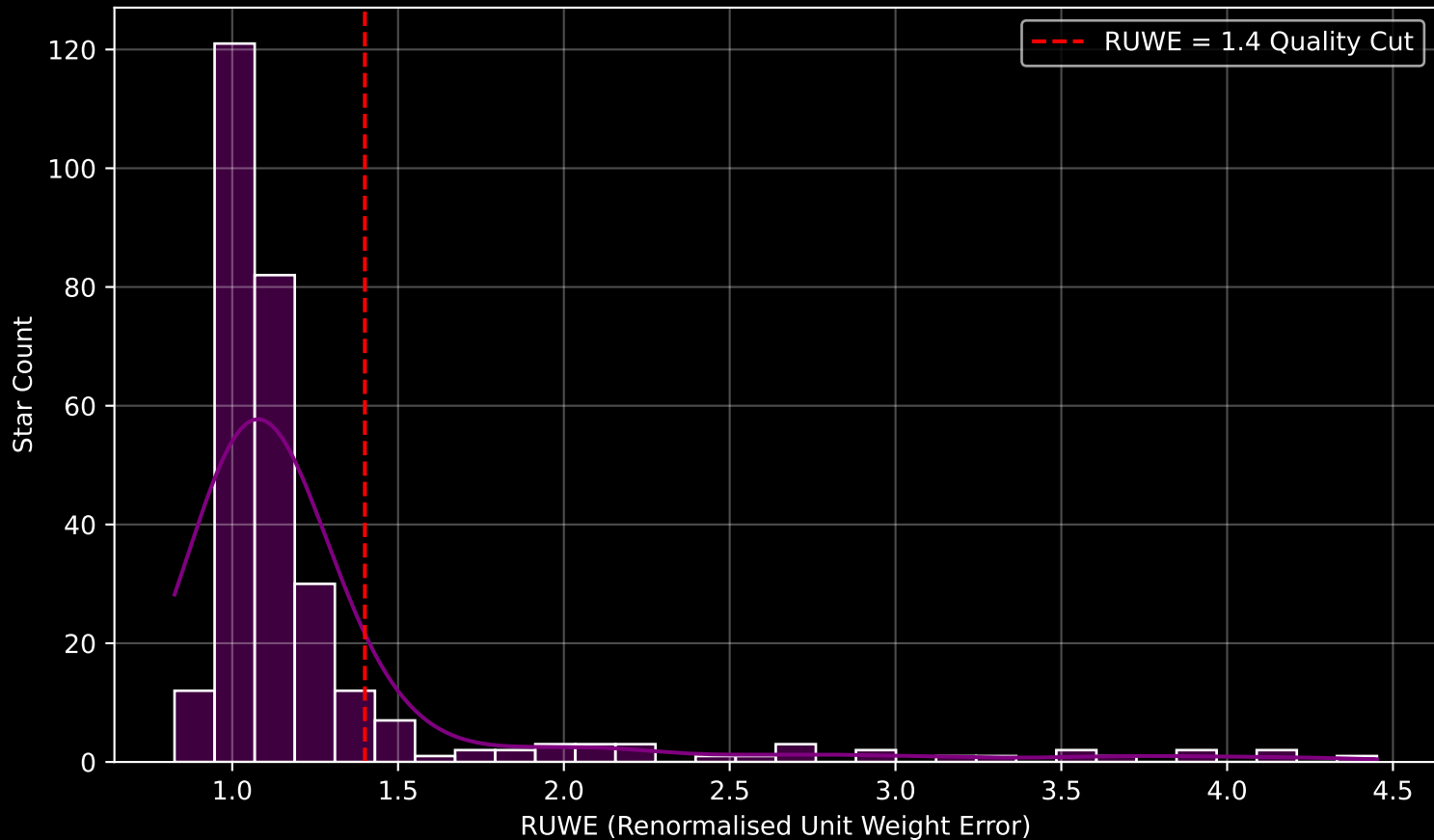
GALAH DR4 Field [7029] RUWE Distribution (n= 295)
