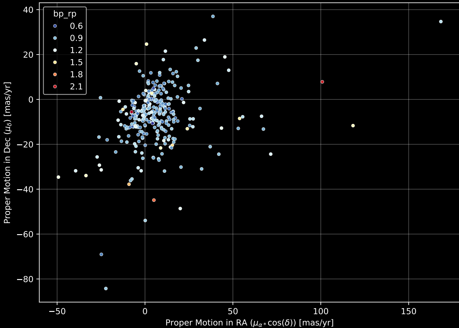
GALAH DR4 Field: [7029] Proper Motion Diagram (n= 300)
