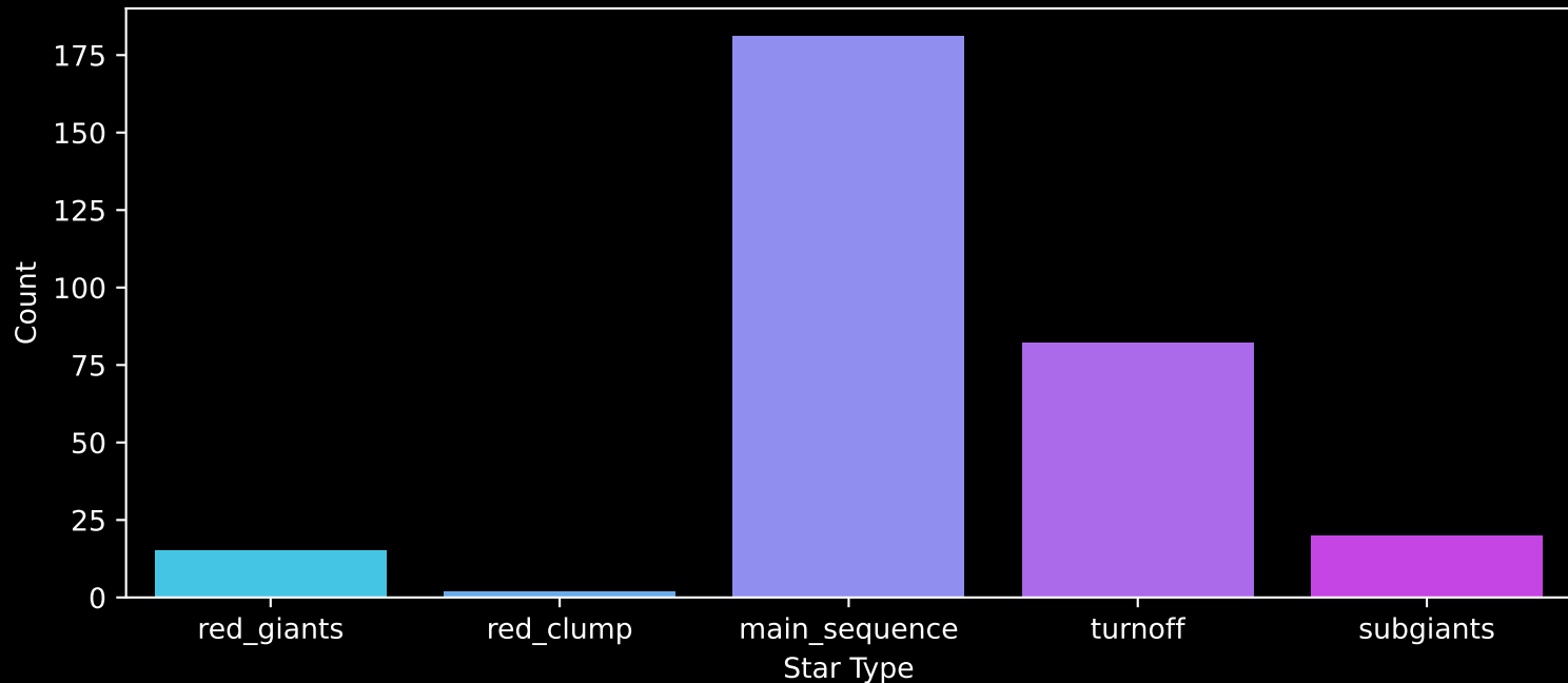
GALAH DR4 Field: [7029] Count plot of Star Type
