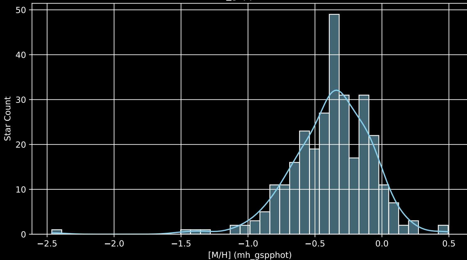
GALAH DR4 Field: [7029] [M/H] (mh_gspphot) (n= 298)
