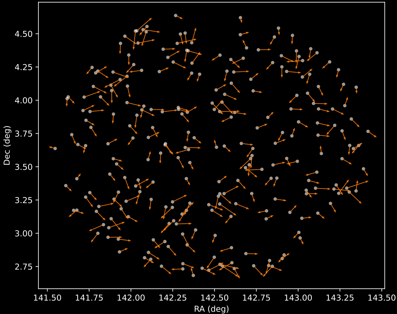
GALAH DR4 Cluster 2 Proper Motion Vectors (n=250)
